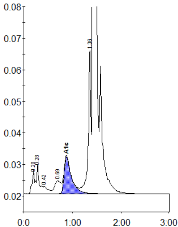
Peak table - ID: 10462232
